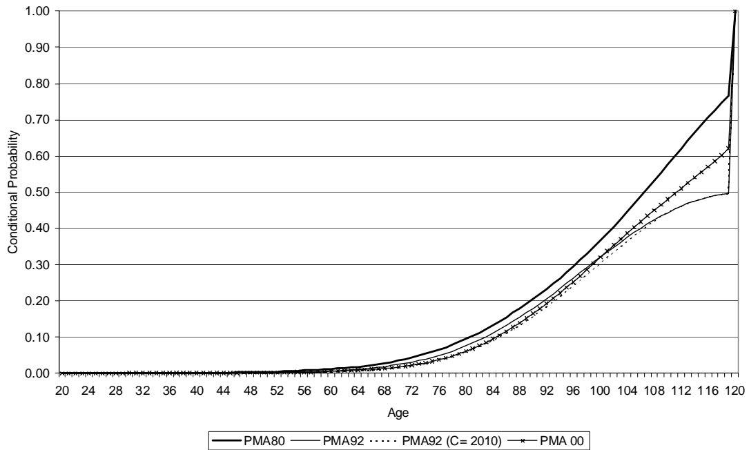
Figure 1: The figure plots the conditional death probabilities for different sets of mortality assumptions. PMA80 reflects the mortality probabilities calculated using data for 1979-1982, PMA92 does the same for 1991-1994 data, and PMA00 for 1999-2002 data. PMA92 (C=2010) is based on the PMA92 data but it assumes improvements in life-expectancy up to 2010.
